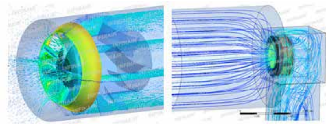
CFD flow field trace of a certain new box-type centrifugal fan of INFINAIR (process illustration)
